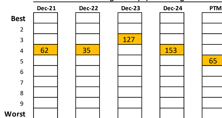
SENX: EPS growth (%) & ranking
